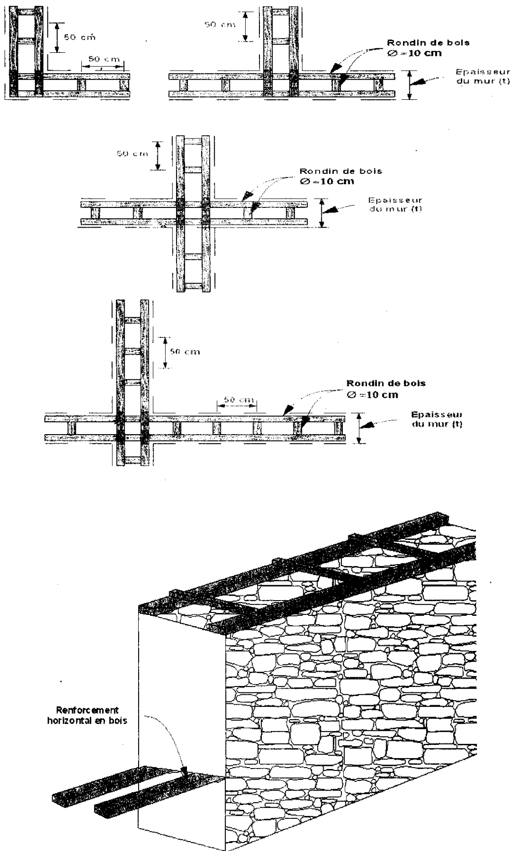
Fig.34. Renforcement horizontal
