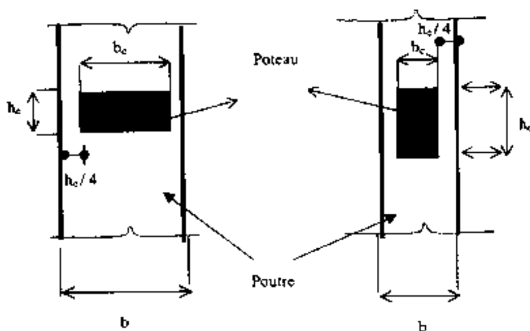
Figure 7.2 : Position poteau-poutre
