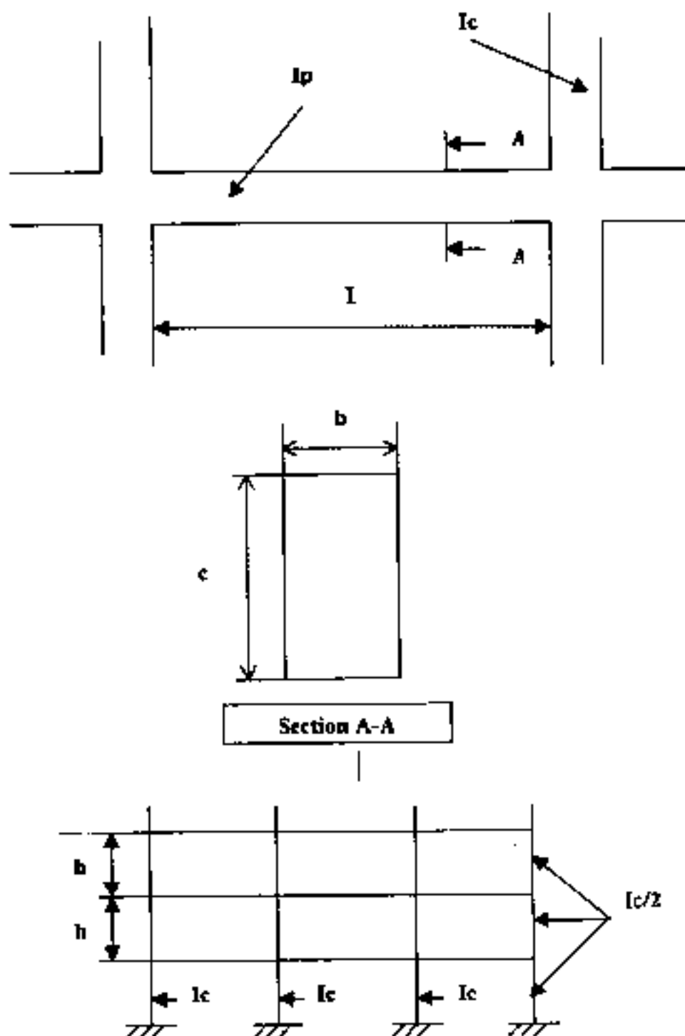
Figure 6.2 : Poutres - Poteaux
